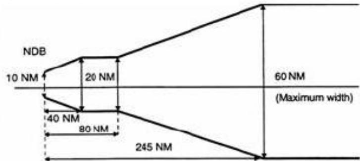
Figure 2: Corridor width from an NDB
