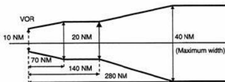
Figure 1: Corridor width from a VOR station
